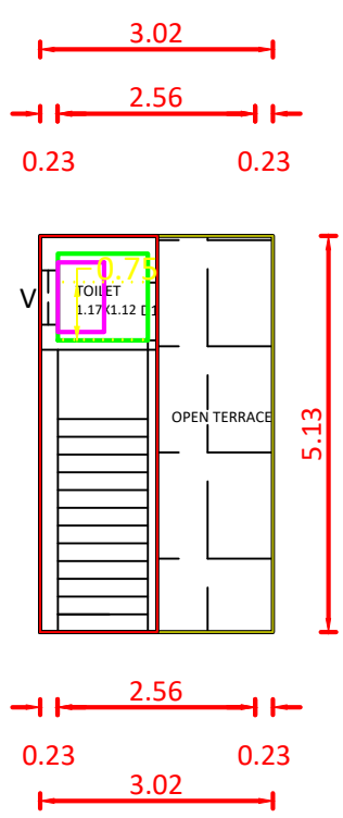
HEAD ROOM PLAN
