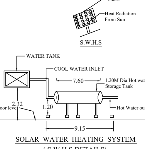
SOLAR WATER HEATING SYSTEM (S.W.H.S.DETAILS)
