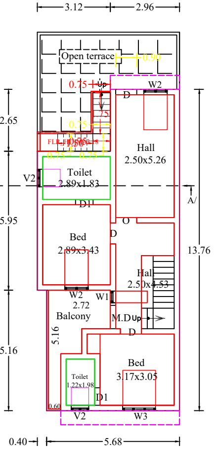
EXTENSION FIRST FLOOR PLAN
