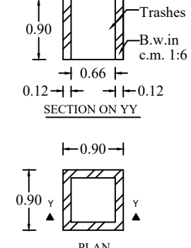
WASTE TRASH PIT
