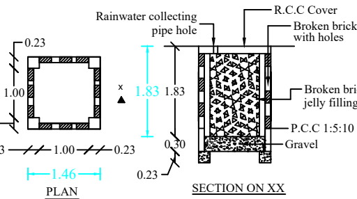
RAIN WATER HARVEST WELL
