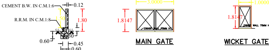
MAIN GATE
