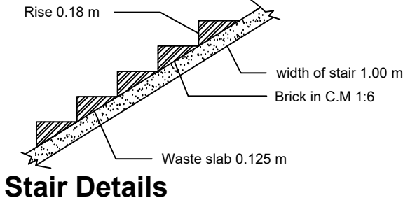
Stair Details
