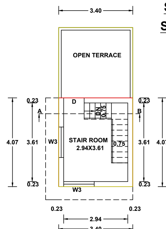
HEAD ROOM PLAN
