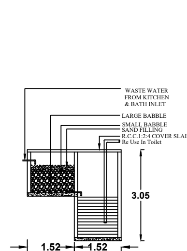
RECYCLING OF WASTE WATER FROM KITCHEN & BATHROOM
