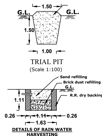
DETAILS OF RAIN WATER HARVESTING
