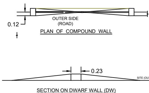
SECTION ON DWARF WALL (DW) (NOT TO SCALE)
