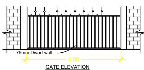
GATE ELEVATION
