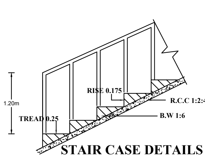
STAIR CASE DETAILS
