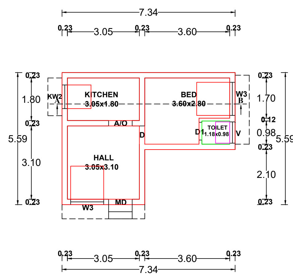
GROUND FLOOR PLAN (BLOCK - 2)
