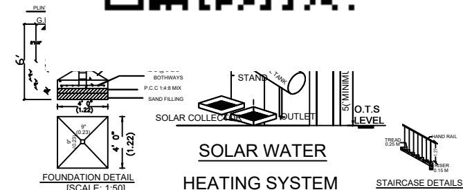
HEATING SYSTEM
