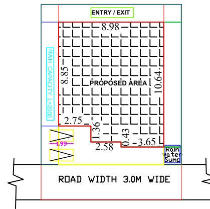
SITE PLAN
