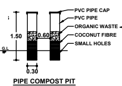
PIPE COMPOST PIT
