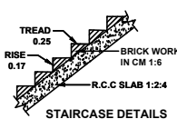
STAIRCASE DETAILS
