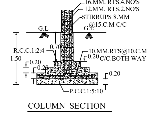
COLUMN SECTION
