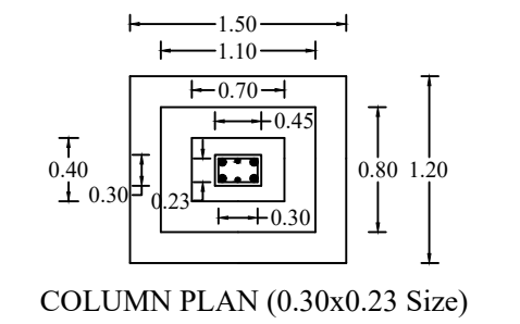
COLUMN PLAN (0.30x0.23 Size)
