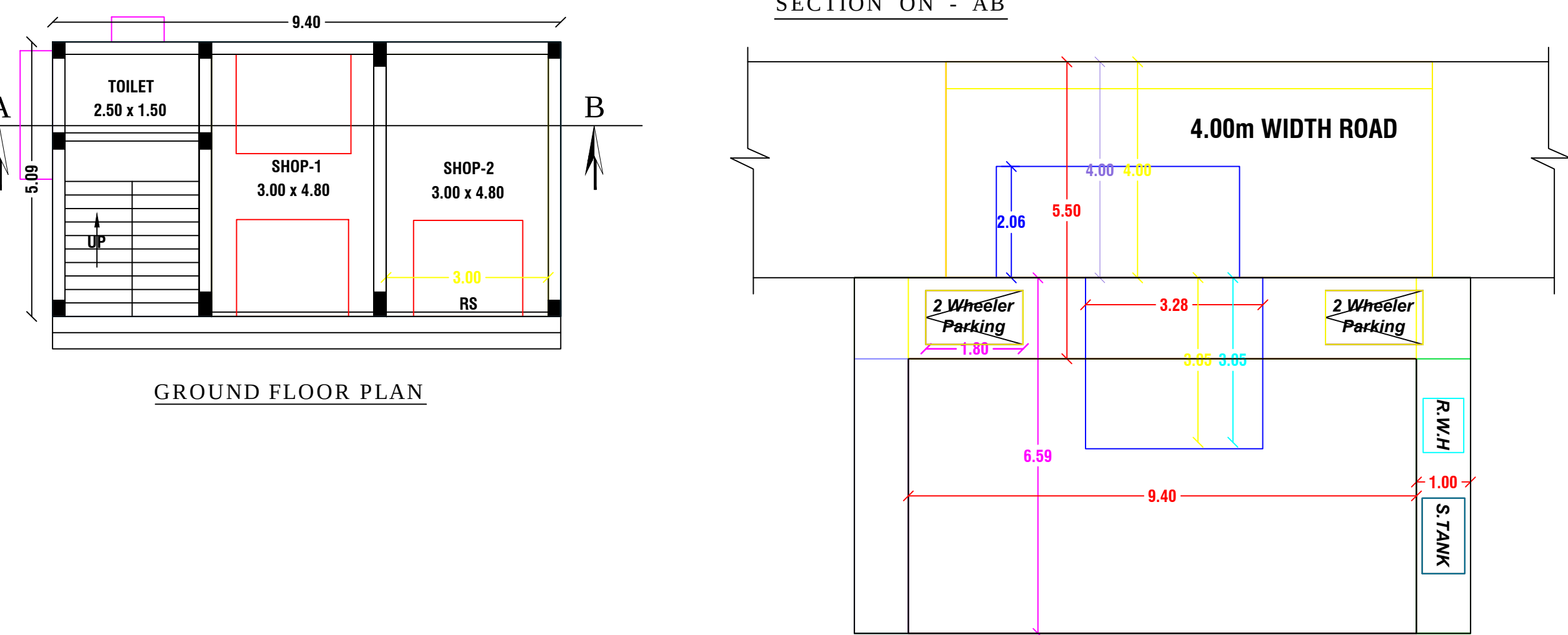
SITE PLAN
