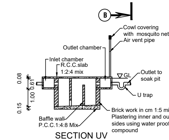
SECTION UV
