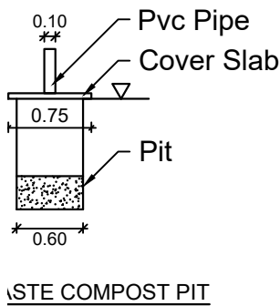
STE COMPOST PIT
