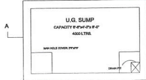
SUMP PLAN
