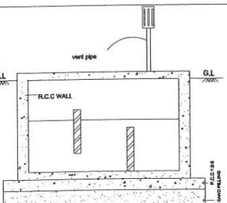
SECTION ON BB
