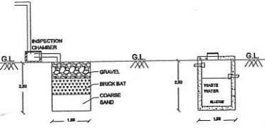
RAIN WATER HARVESTOR
