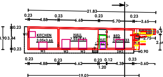
FIRST FLOOR PLAN SCALE: 1: 100
