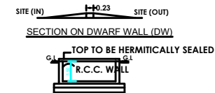
RWH SECTION (SAMPLE) RWH_CAPACITY_L=4800LTRS
