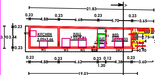
GROUND FLOOR PLAN SC
