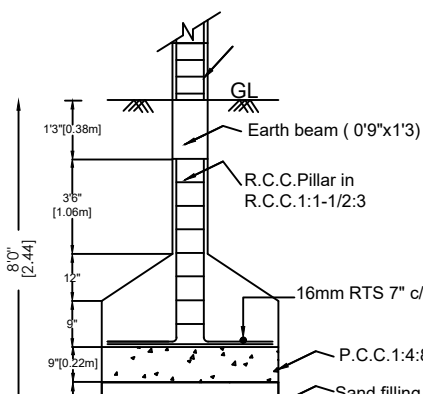
FOUNDATION DETAILS
