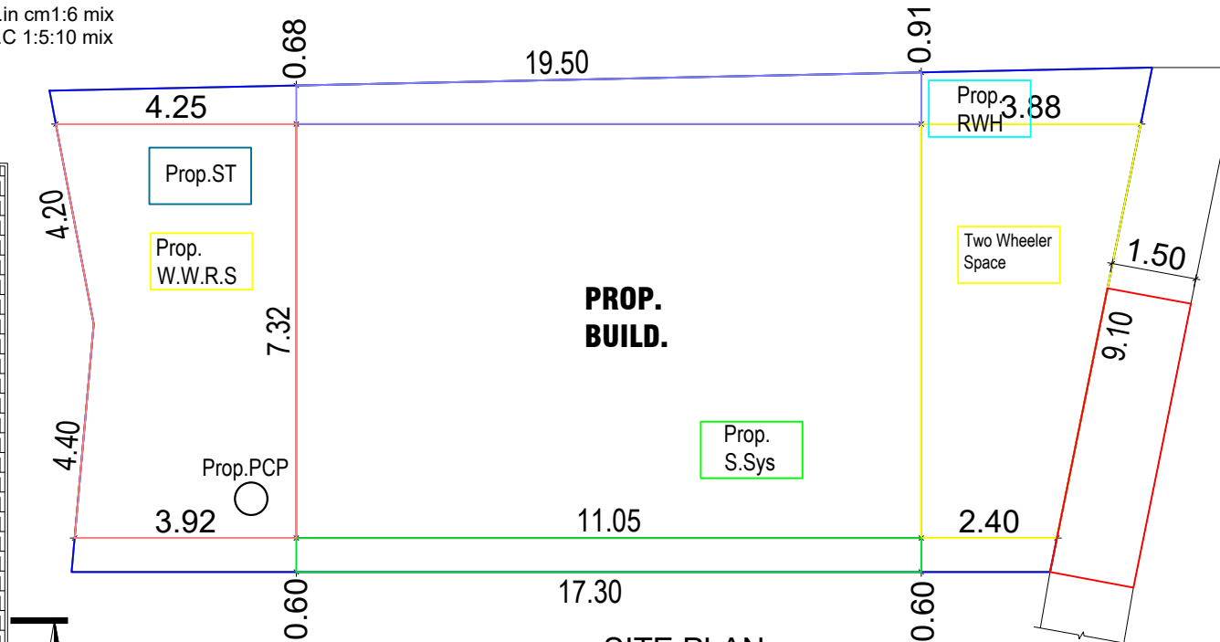
SITE PLAN
