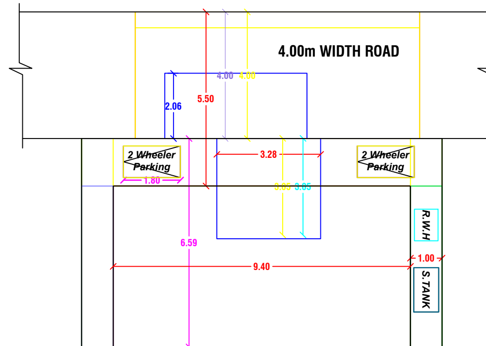
SITE PLAN
