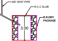
SECTION OF SOAKPIT
