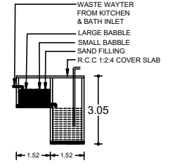
RECYCLING OF WASTE WATER TANK
