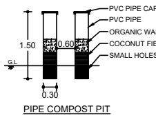
PIPE COMPOST PIT
