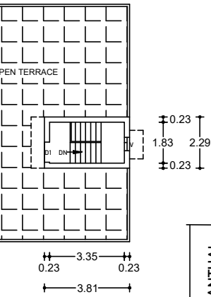
FLOOR PLAN
