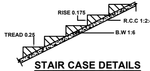
STAIR CASE DETAILS
