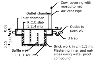
SECTION UV
