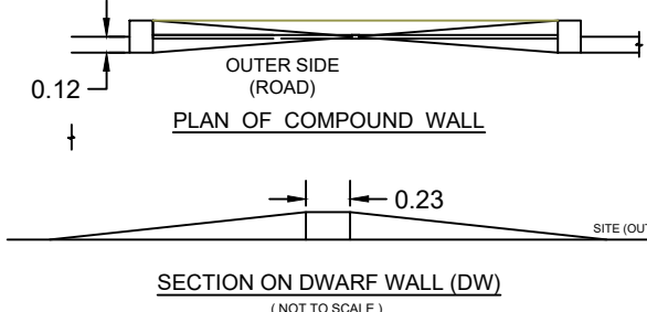
PLAN OF COMPOUND WALL
