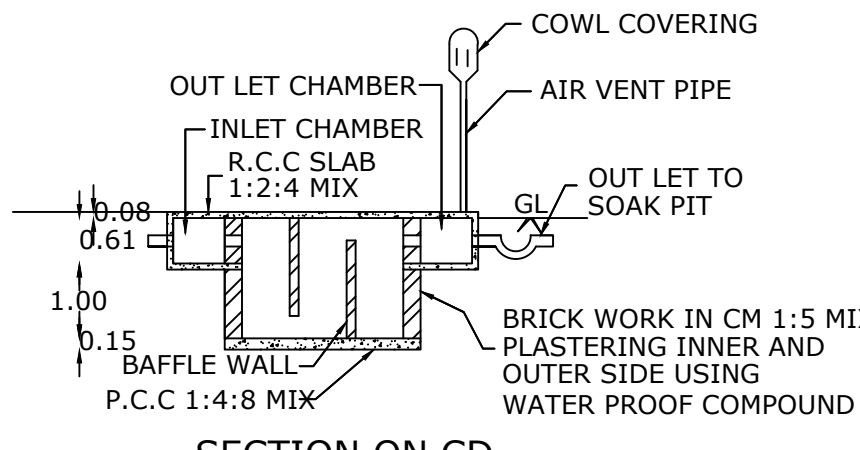
SECTION ON CD
