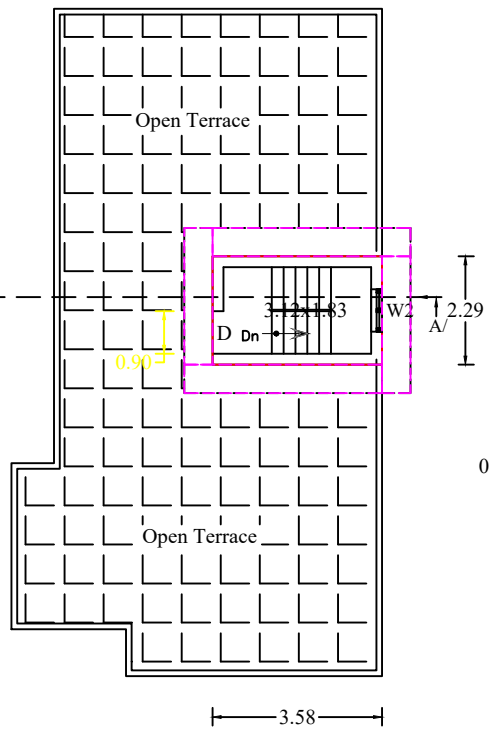
HEAD ROOM PLAN
