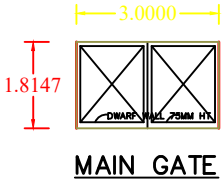
MAIN GATE
