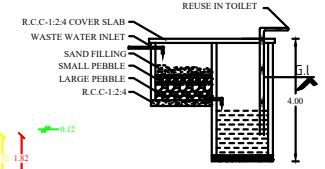
RECYCLING OF WASTE WATER KITCHEN & BATH ROOM
