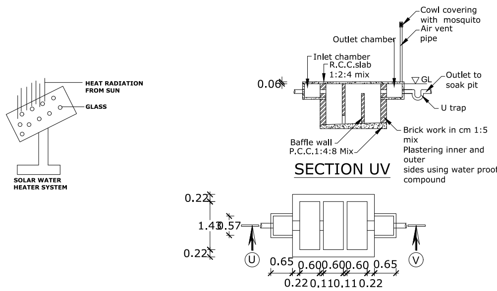
RECYCLING OF WASTE WATER SYSTEM
