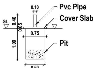
WASTE COMPOST PIT
