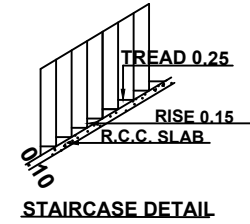
STAIRCASE DETAIL
