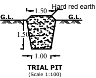
TRIAL PIT
