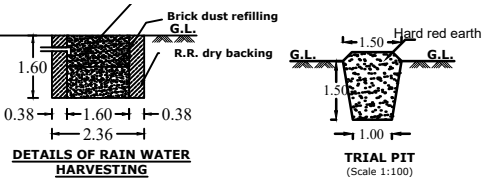
DETAILS OF RAIN WATER HARVESTING
