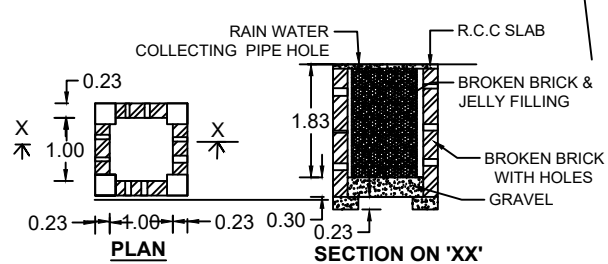
RAIN WATER HARVEST WELL
