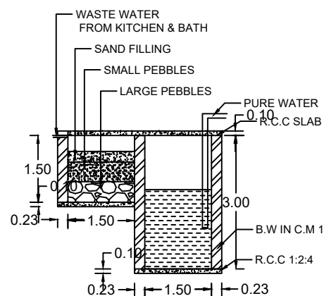
WASTE WATER RECYCLING SYSTEM
