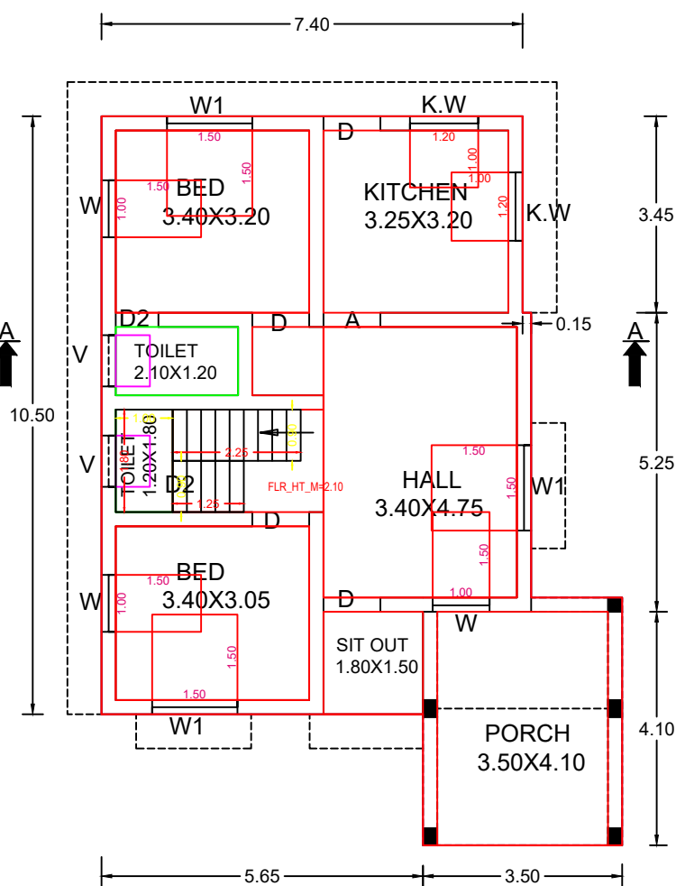
G.F. PLAN
