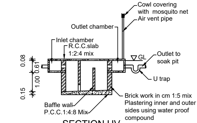
SECTION UV
