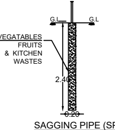
SAGGING PIPE (SP)
