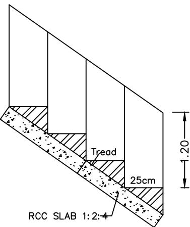
STAIR DETAILS
