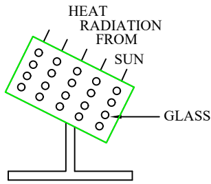
SOLAR SYSTEM
