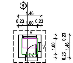
SECTION ON ST
