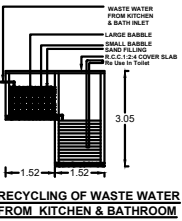
RECYCLING OF WASTE WATER FROM KITCHEN & BATHROOM
