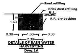
DETAILS OF RAIN WATER HARVESTING Dwg: 1A
