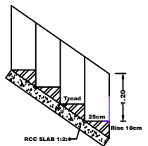
STAIR DETAILS
