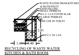
RECYCLING OF WASTE WATER KITCHEN & BATH ROOM
