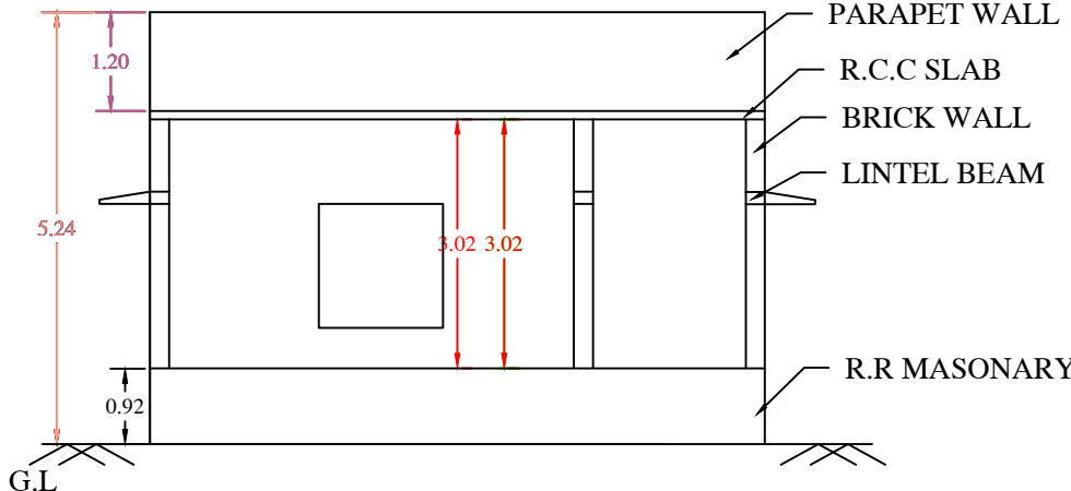
SECTION AT X-X'
