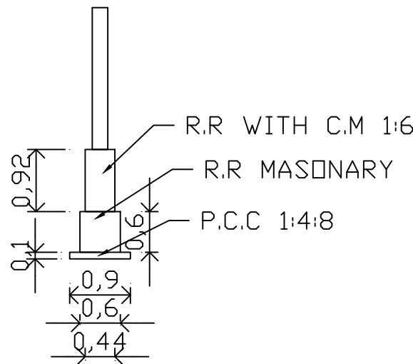
FOUNDATION
