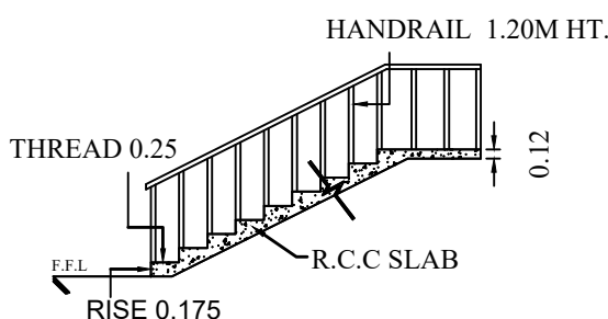
STAIRCASE DETAILS
