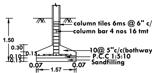
SECTION OF COLUMN
