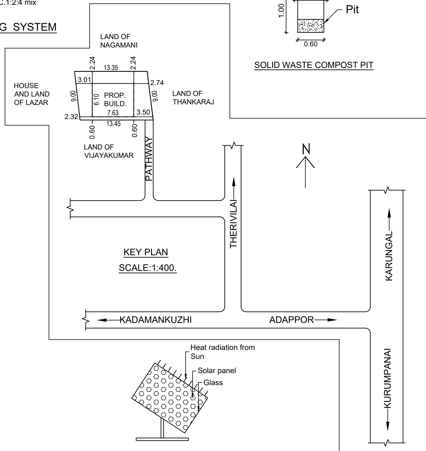
SOLAR SYSTEM
