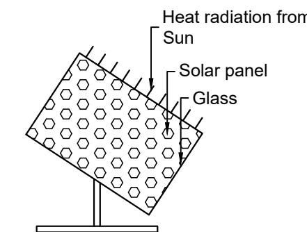
SOLAR SYSTEM
