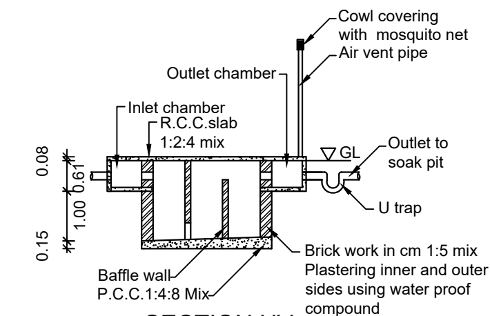
SECTION UV
