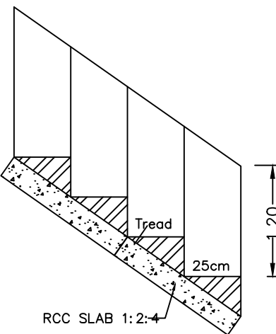
STAIR DETAILS
