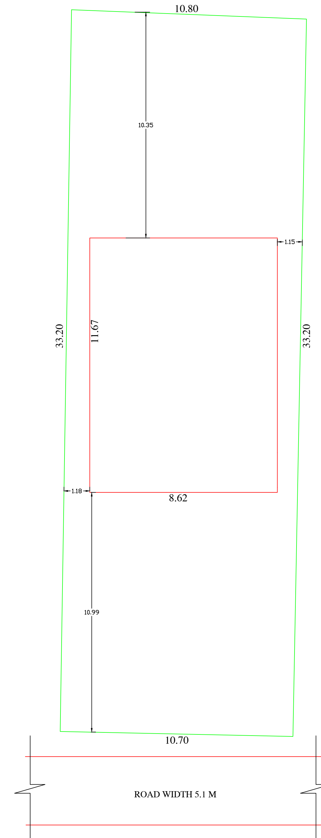
SITE PLAN
