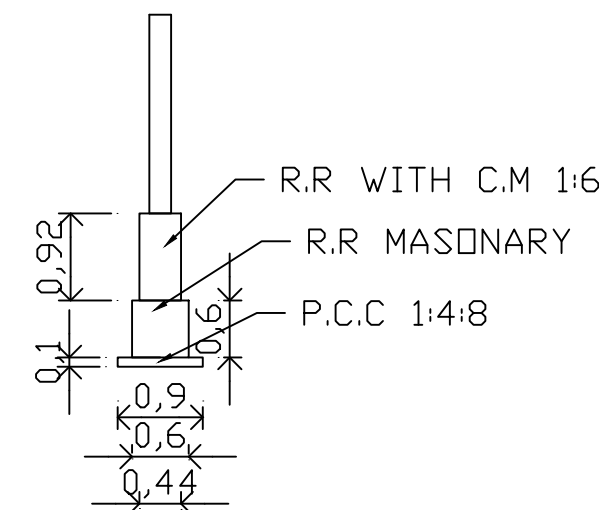
FOUNDATION
