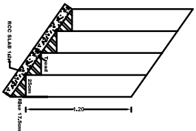
STAIR DETAILS
