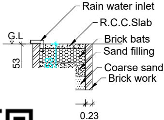
DETAIL OF RAIN WATER INLET DETAIL OF RAIN WATER INLET
