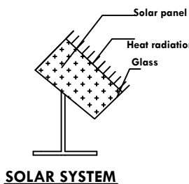
SOLAR SYSTEM
