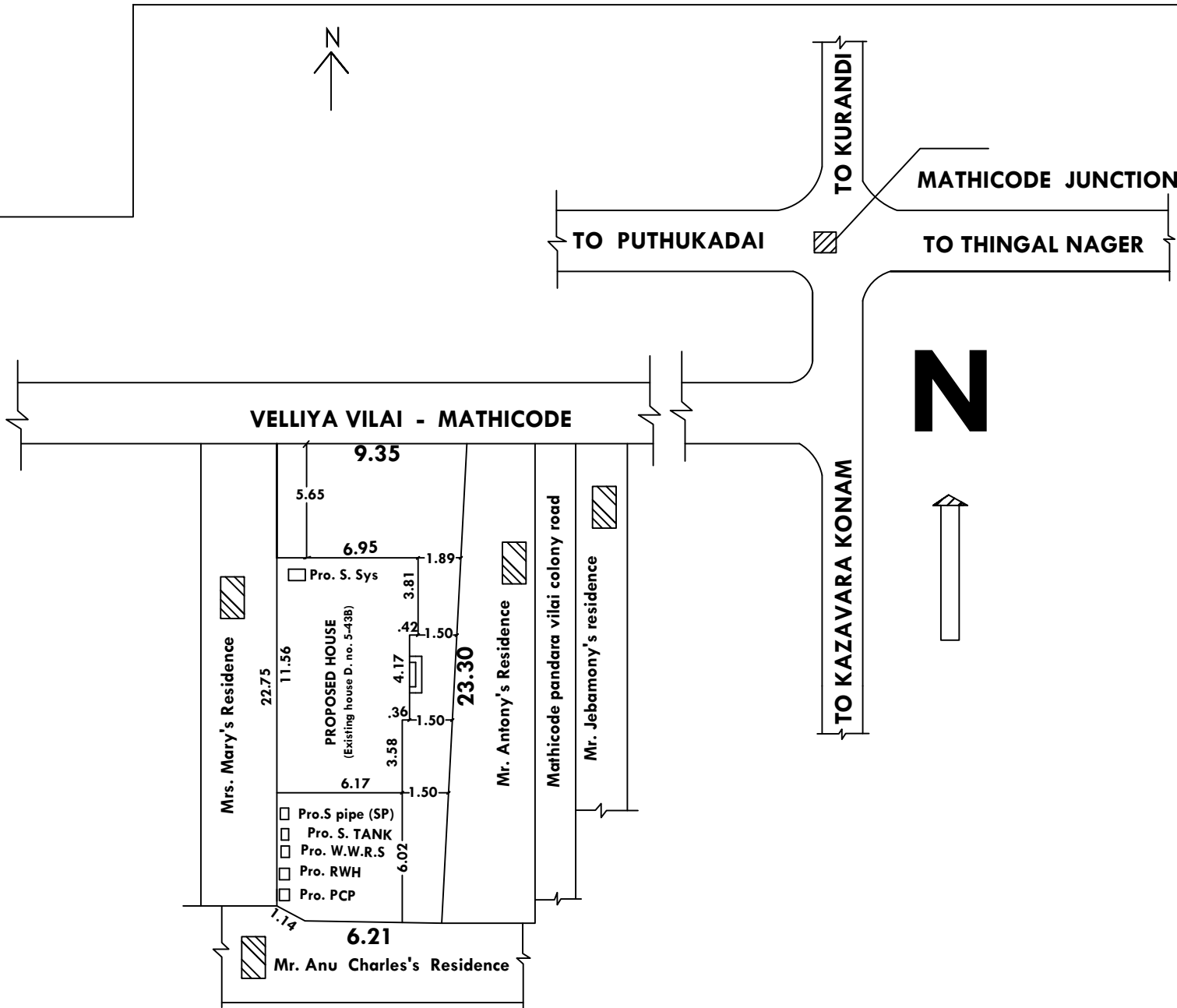
LOCATION PLAN (NOT TO BE SCALE)
