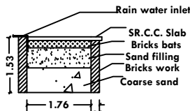
RAIN WATER HARVESTING TANK RWH CAPACITY 5000 LTRS
