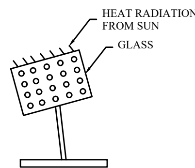
SOLAR SYSTEM
