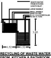
RECYCLING OF WASTE WATER FROM KITCHEN & BATHROOM
