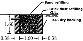
DETAILS OF RAIN WATER HARVESTING
