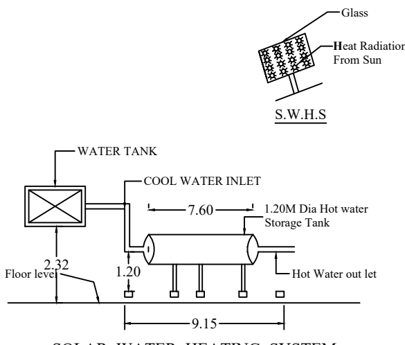
SOLAR WATER HEATING SYSTEM (S.W.H.S.DETAILS)
