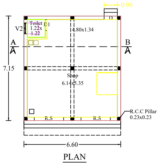
PLAN
