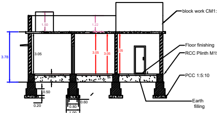
SECTION ON A-B [1:100]
