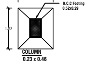
SECTION OF COLUMN
