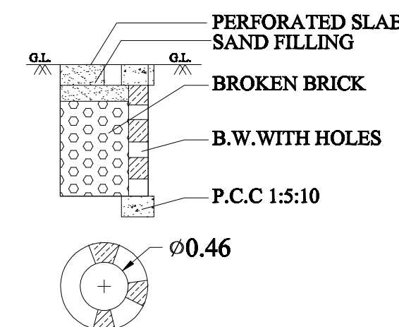
RAIN WATER PERCOLATION DRAWING TYPE -1A
